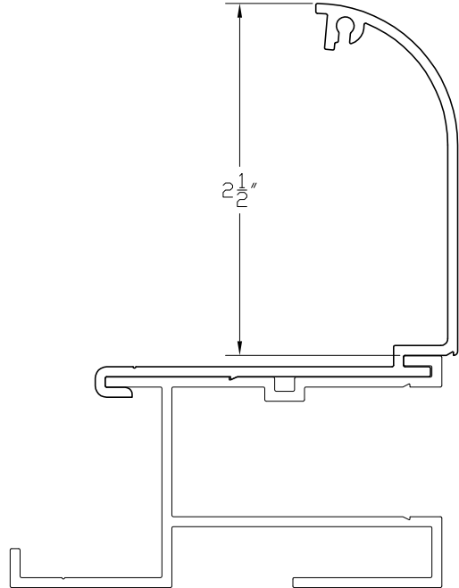
Rounded Clip-on Coping
