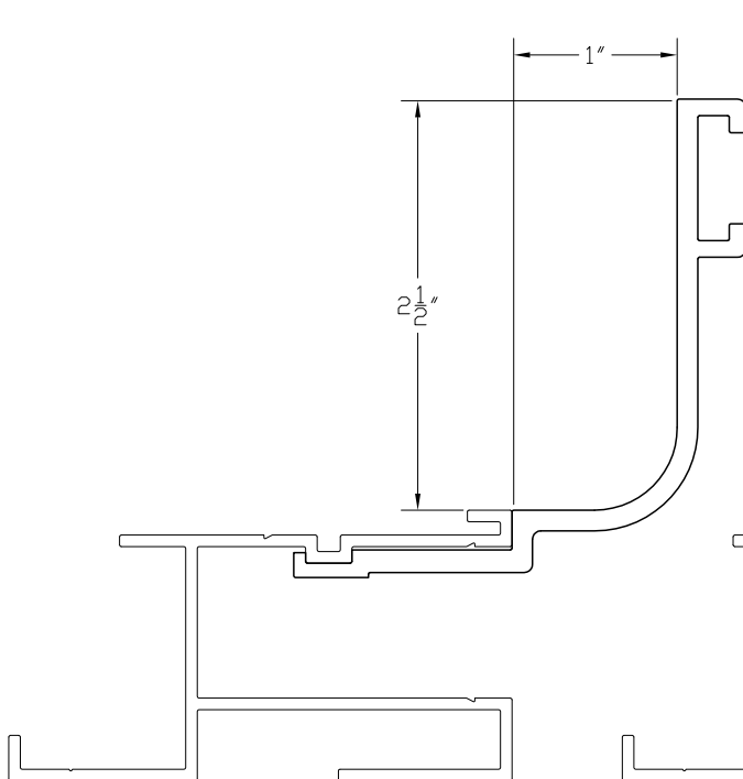
Cantilever Reusable Form
