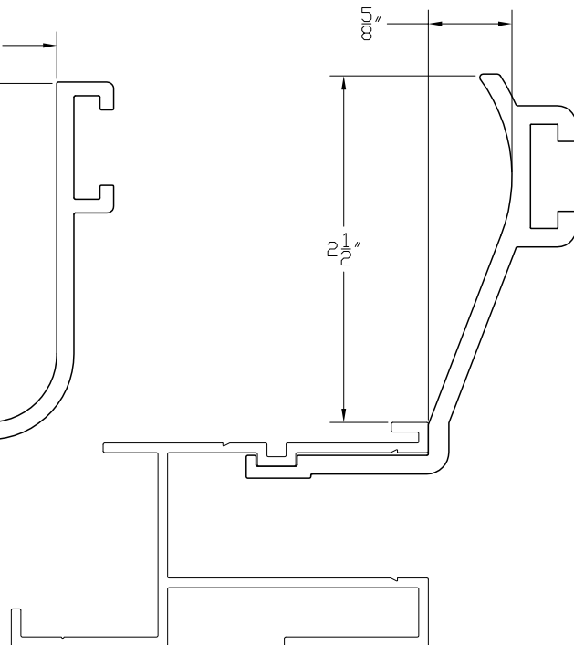
Inclined Reusable Form
