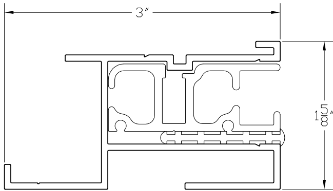
Fiberglass Encapsulation
